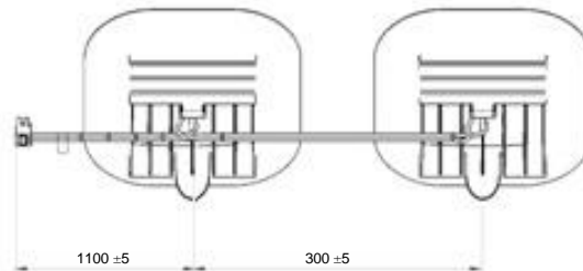
Assembly with cable harness
