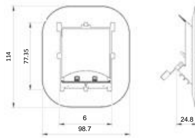
Base plate
